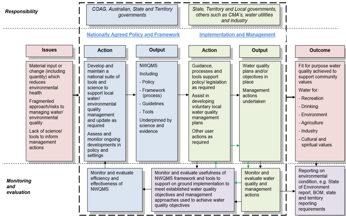
Figure 1: NWQMS logic
